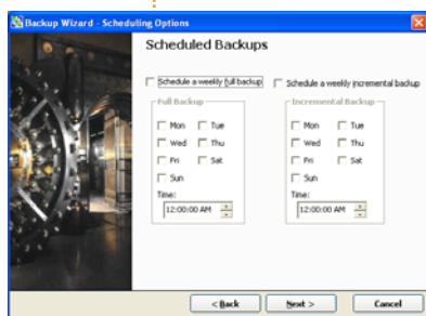
Backup Scheduler
