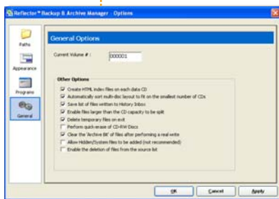
Options Screen
