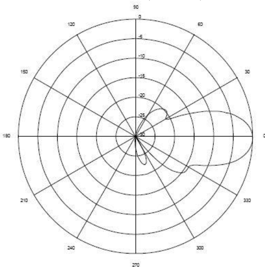
RF Patterns (Vertical)
