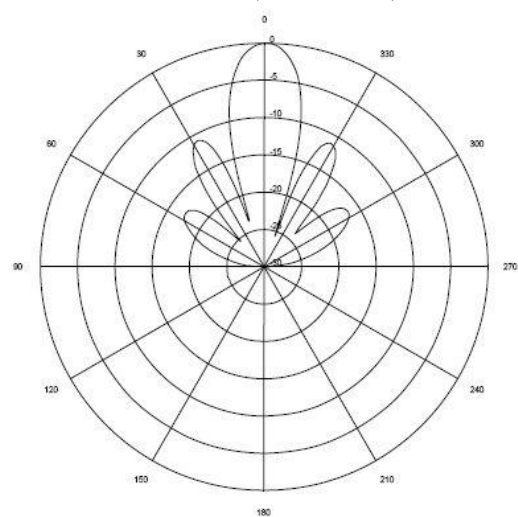
RF Patterns (Horizontal)
