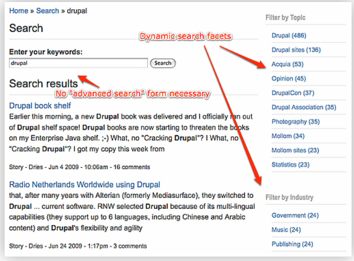
Acquia Search Interface
