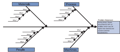
Ishikawa Diagram
