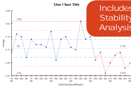
Control Chart
