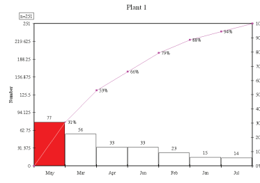
Pareto Chart
