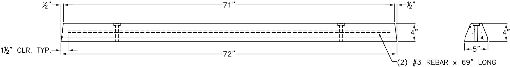
SIDE-VIEW
