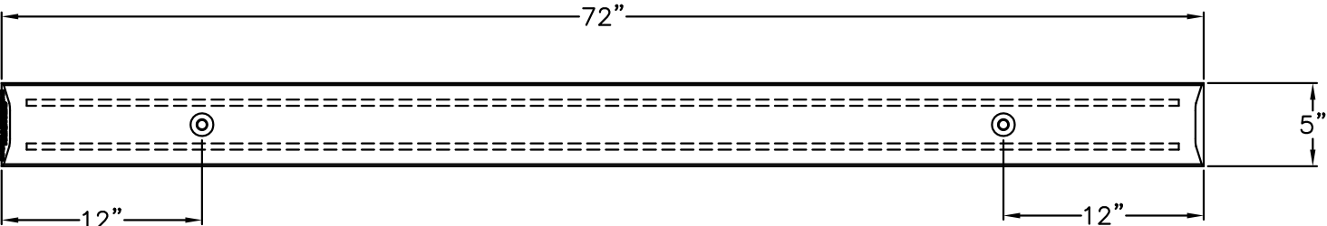
TOP-VIEW
