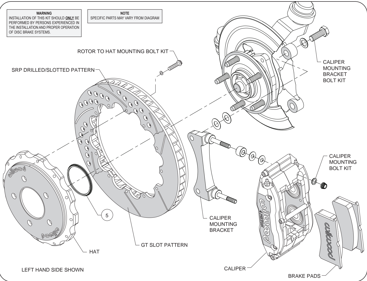
Typical Installation Diagram • Part Number 140-12440 / -D
