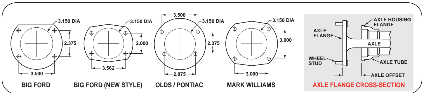
Rear Housing Flange Chart and Axle Flange / Offset Cross-Section
