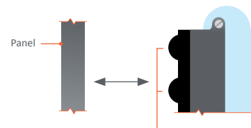
Custom gasket with dual compression rings
