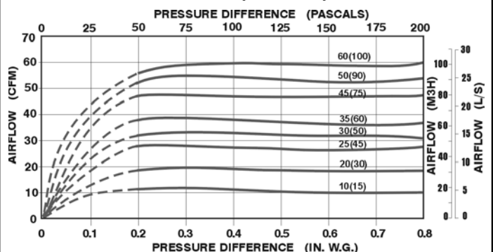
ZRT-1-4 or ZRT-2-4 MAXIMUM FLOW CONTROL ZRT-2-6 MINIMUM FLOW CONTROL 4" DIA. (100mm)
