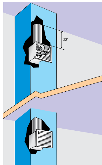
Example: ZRT-2 installed in a central ventilation duct riser
