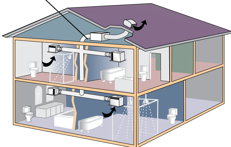
Example: ZRT-1 multi-zone central ON/OFF ventilation system
