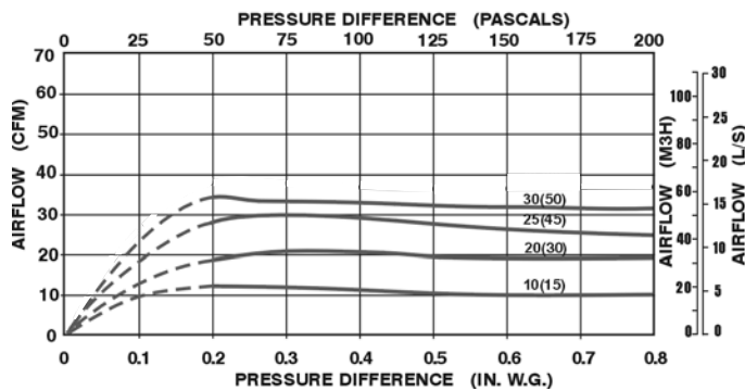
ZRT-2-4 MINIMUM FLOW CONTROL 3" DIA. (80mm)
