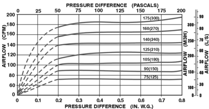
ZRT-1-6 or ZRT-2-6 MAXIMUM FLOW CONTROL 6" DIA. (150mm)
