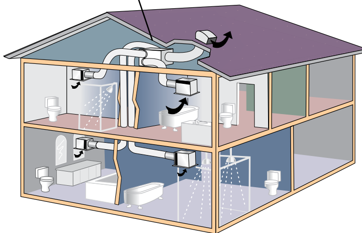
Example: ZRT-2 low continuous with no-limit maximum-boost ventilation control
