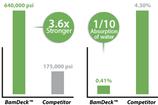
Strength Test Modules of Elasticity (ASTM D4761)
