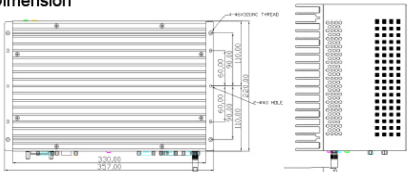
Dimension
