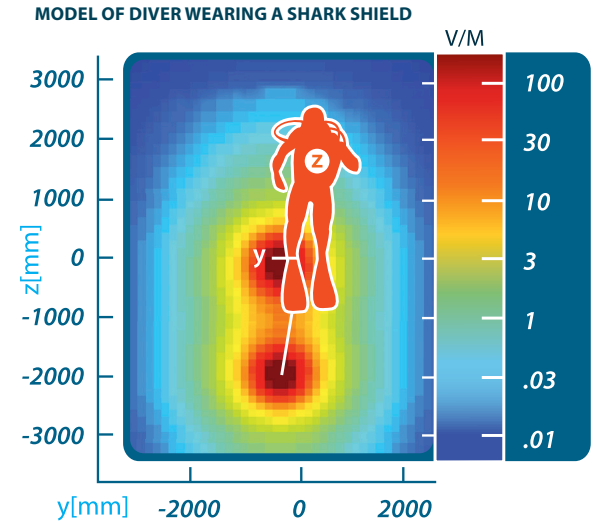
SANSA 2012: Estimated magnitude of the E-field surrounding a model of a diver wearing Shark Shield
