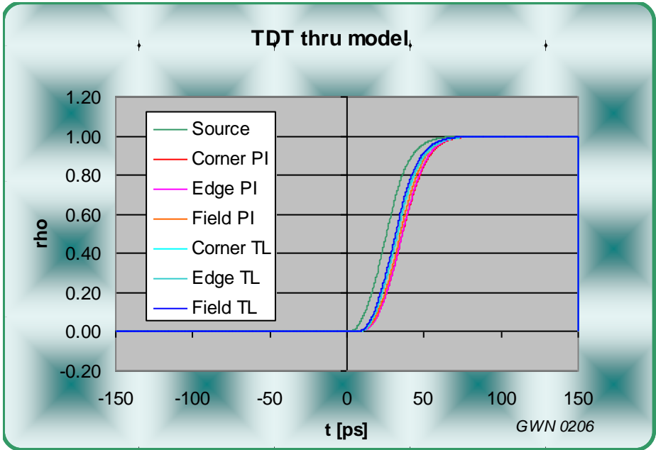
Figure 33 TDT model
