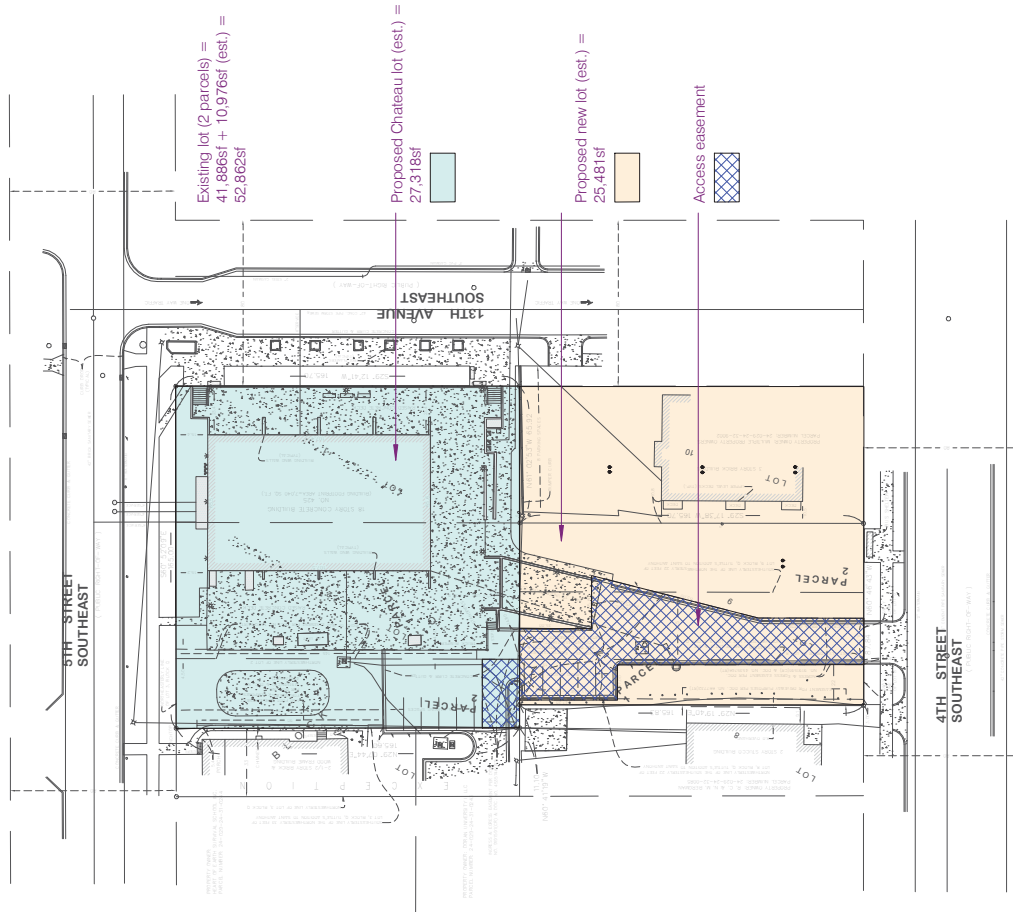
1 Proposed site division
