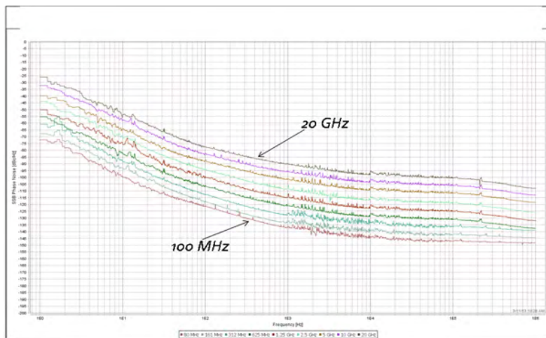
Phase Noise Performance (1 Hz to 50 MHz offset)
