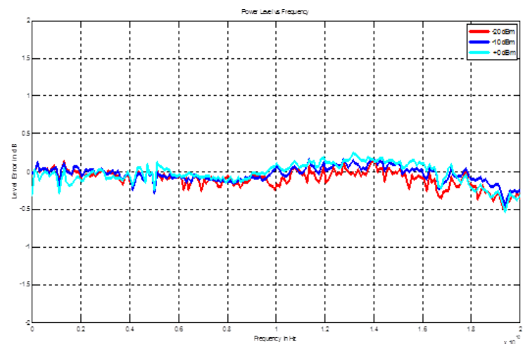
Typical Frequency Response 0 to 20 GHz at -10, 0, and +10 dBm
