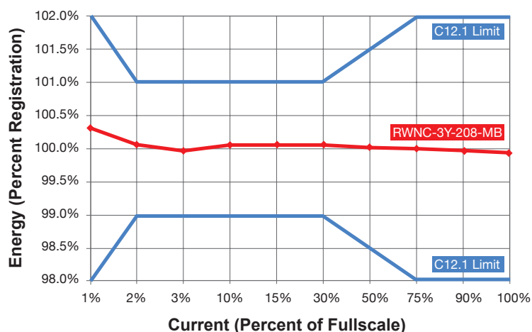
ANSI C12 Load Performance Test - RWNC-3Y-208-MB WattNode Revenue
