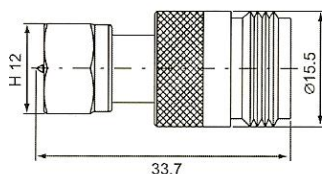
F male - N female FN-312 (75 Ω)
