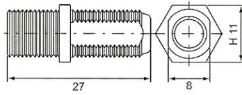
F female Bulkhead receptacle F-332-27 D/D (75 Ω)
