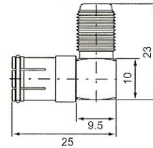
Double F female right angle F-422(75 Ω)
