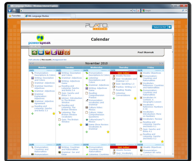
Learner Interface
