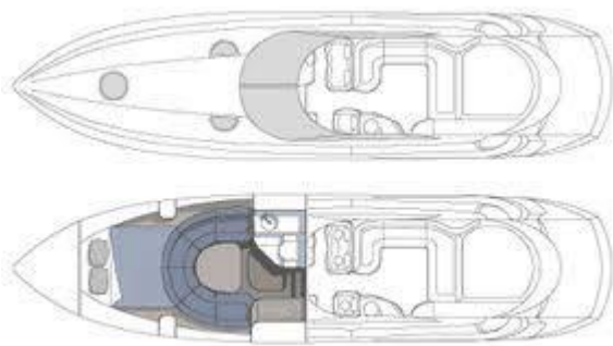
Sunseeker Superhawk 34 Layout
