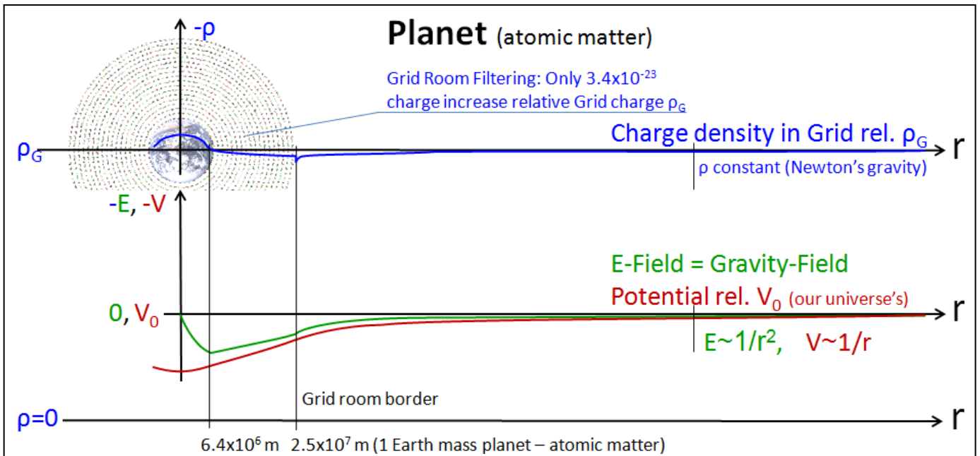
Figure 17: Illustration of the charge density, the gravity field and the electric potential in and around a planet. Planets consist of atomic matter and the diagram is similar to Figure 15. The size calculations in this and the following figures are based on that the contribution from the Grid room always is 96.4 \text{ kg/m}^3 (as shown in ToS 4.5.3), which makes up the mass of the object encapsulated by the Grid room.
