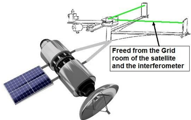
Figure 13: A modified Michelson–Morley interferometer on a satellite will show that the speed of light varies when the satellite is moving in the Grid. It is important that the traces between the mirrors are not in the Grid room of the satellite or in the Grid room of the interferometer itself.
