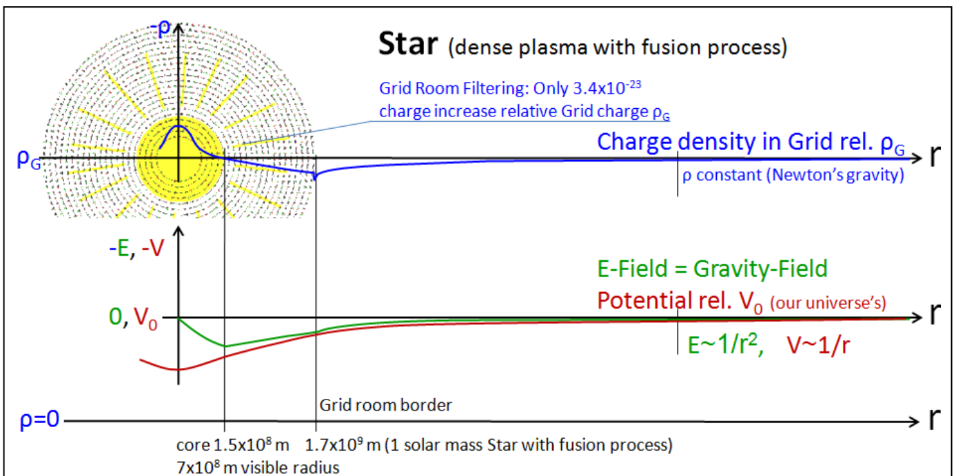
Figure 18: Illustration of the charge density, the gravity field and the electric potential in and around an ordinary star. The core of the star contains plasma of higher density than is possible for atomic matter, and the fusion process upholds the gravity pressure from further compression from the gravity.
