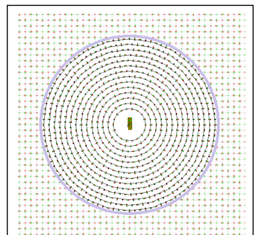
Figure 10: The Grid room of a proton consists of thirteen layers of negtrinos that encapsulate the particle. The particle is stuck in its Grid room – all movements are at the border between the Grid room and the Grid.
