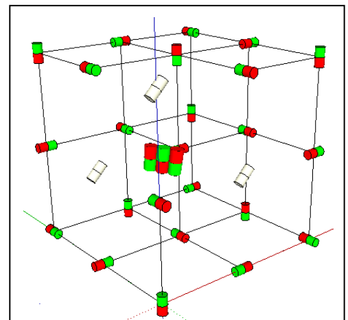
Figure 8: A neutrino consisting of 3 negtrinos pushes off 3 negtrinos in the Grid (white), getting zero visible charge. It does not “take over” any negtrinos in the Grid and therefore shows no mass.
