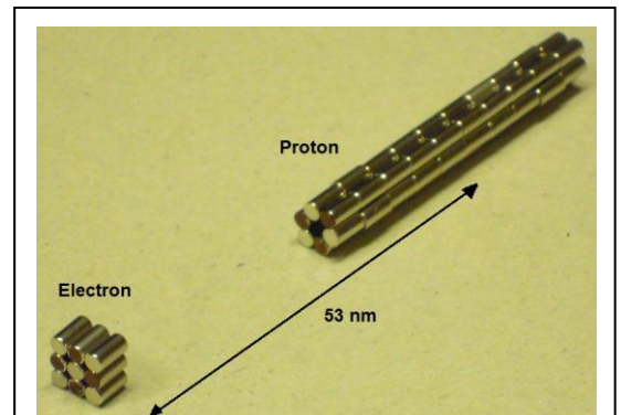
Figure 7: The hydrogen atom built by cylindrical magnets to illustrate the geometry of the proton and the electron. The electron is trapped in a potential well at one of the two poles of the proton and does not have to orbit.
