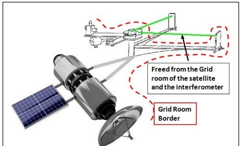
Figure 13: A modified Michelson–Morley interferometer on a satellite will show that the speed of light varies when the satellite is moving in the Grid. It is important that the traces between the mirrors are not in the Grid room of the satellite or in the Grid room of the interferometer itself.
