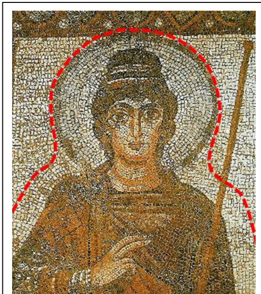
Figure 12: A Grid room surrounds every object. Around a sphere with a density of a human body, its diameter is 2.2 times larger than the sphere, just like the Gloria in this mosaic. The Grid of negtrinos would be arranged similar to the mosaic squares.
