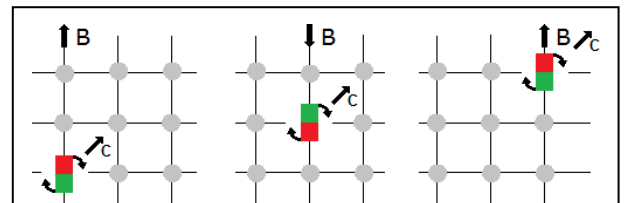
Figure 4: The photon is the energy of a negtrino rotating orthogonally to its spin. The negtrino distance of 10 pm is the wave length separating gamma rays (having shorter wave lengths than 10 pm) from X-rays (having longer wave lengths than 10 pm).
