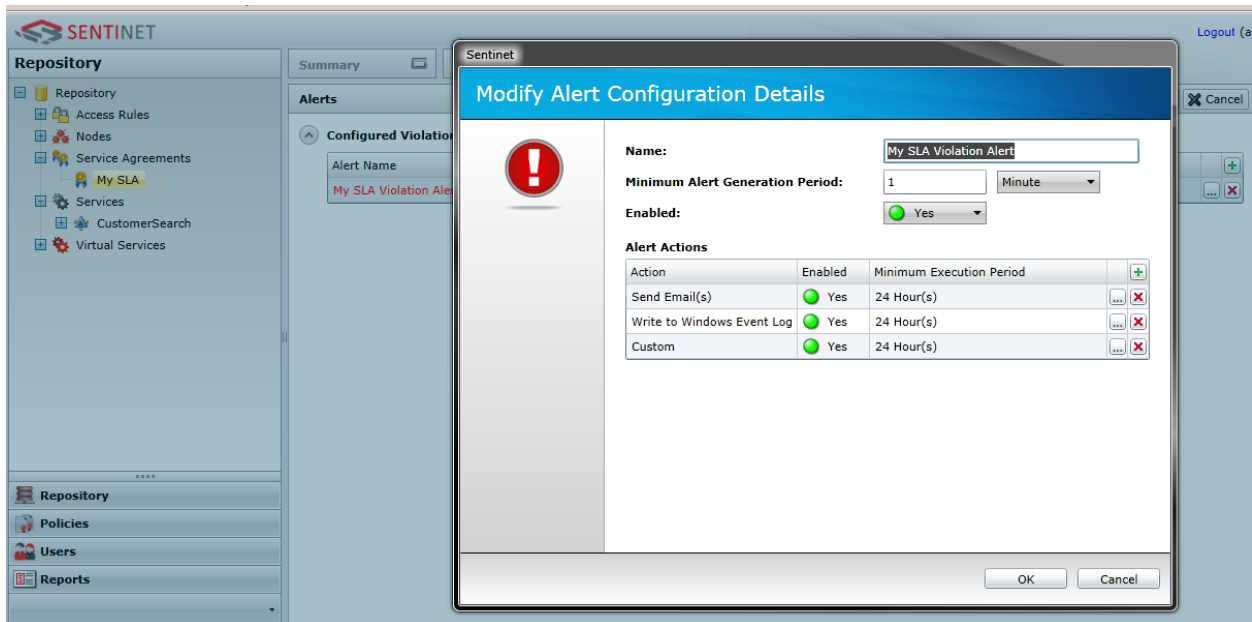
Figure 19. Sample SLA Alert Configuration.
