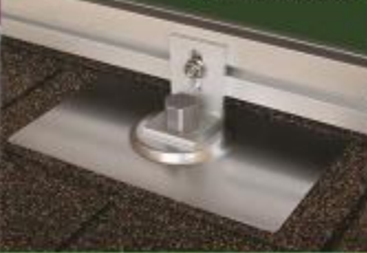
Ez Mount L Foot for Shingle Roofs
