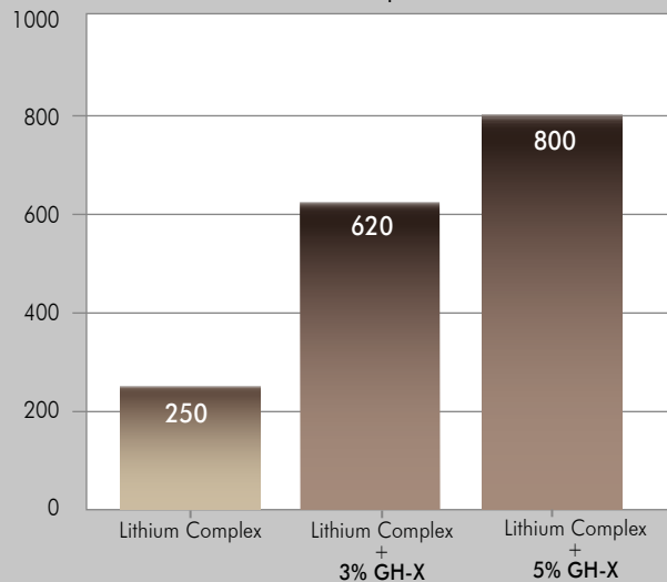
Extreme Pressure Properties Test Results
