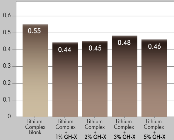
Wear Scar Diameter (WSD) Test Results
