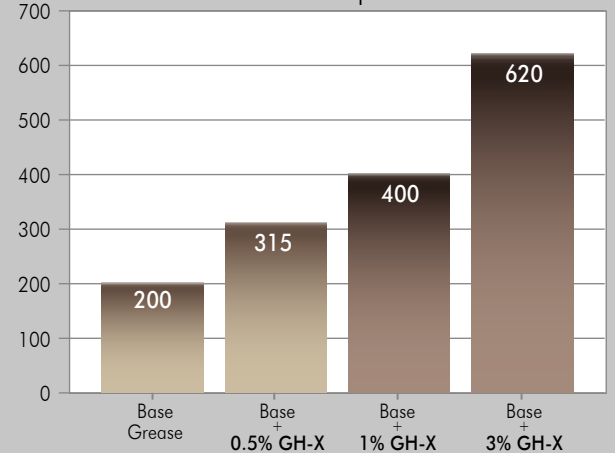
Extreme Pressure Properties Test Results
