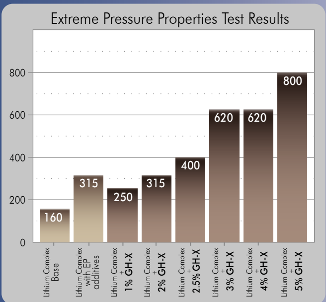
4 Balls EP ASTM 2596
