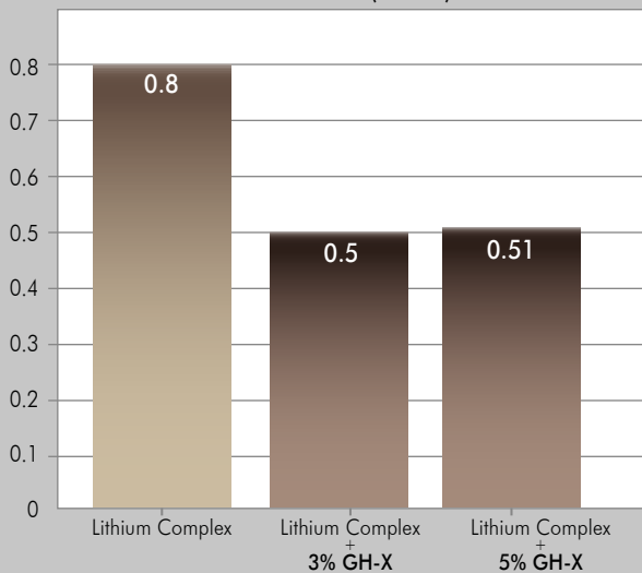
Wear Scar Diameter (WSD) Test Results
