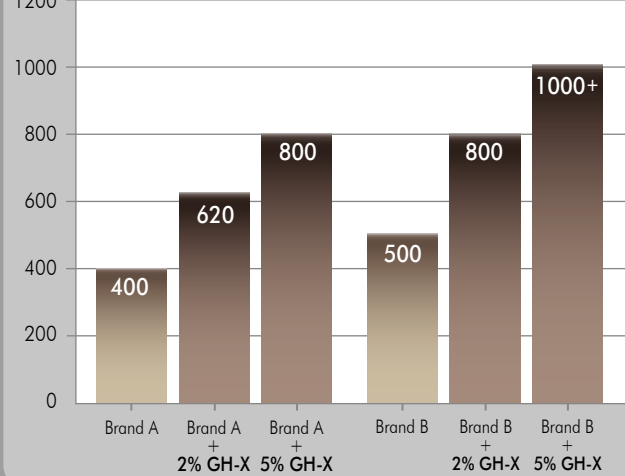
Extreme Pressure Properties Test Results
