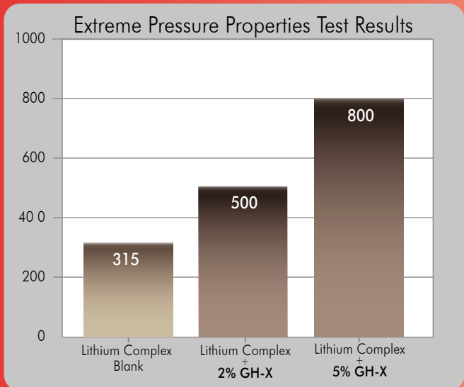
4 Balls EP ASTM 2596
