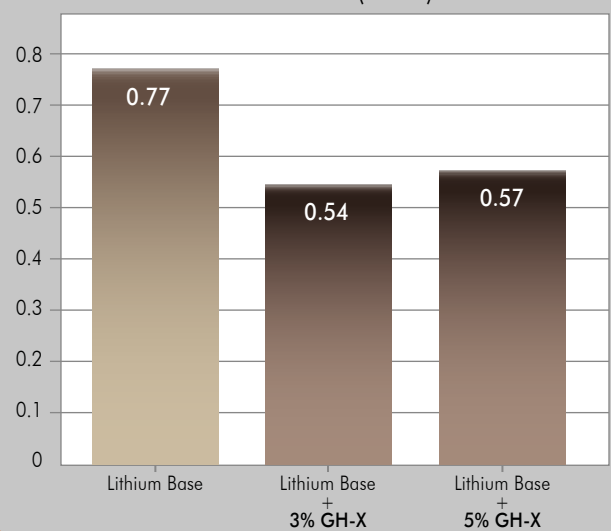
Wear Scar Diameter (WSD) Test Results
