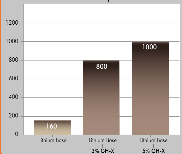
Extreme Pressure Properties Test Results
