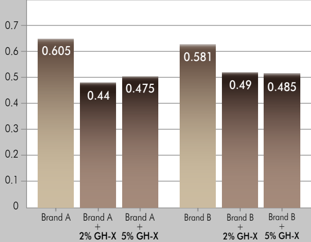
Wear Scar Diameter (WSD) Test Results
