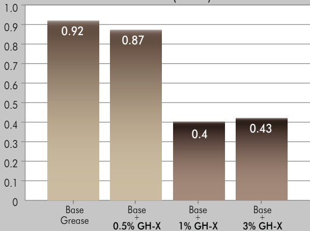
Wear Scar Diameter (WSD) Test Results
