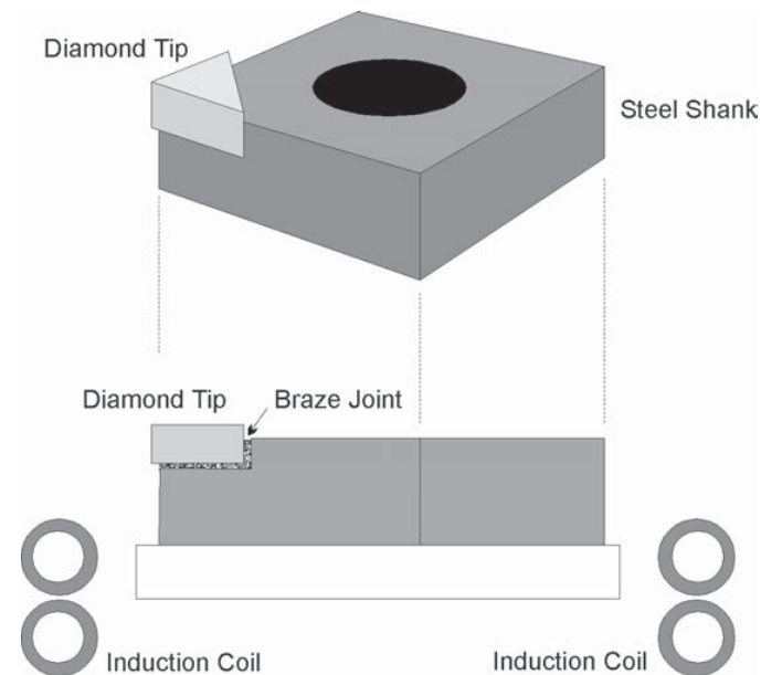
Figure 4: Diamond tips are brazed to the corners of steel shanks for high-speed machine tools.
