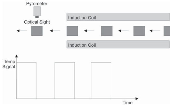
Figure 10: The peak picker mode of the infrared pyrometer picks the "peak" temperature of each part and controls the power supply to maintain the part temperature at 900^{\circ} \pm 10^{\circ}F .
