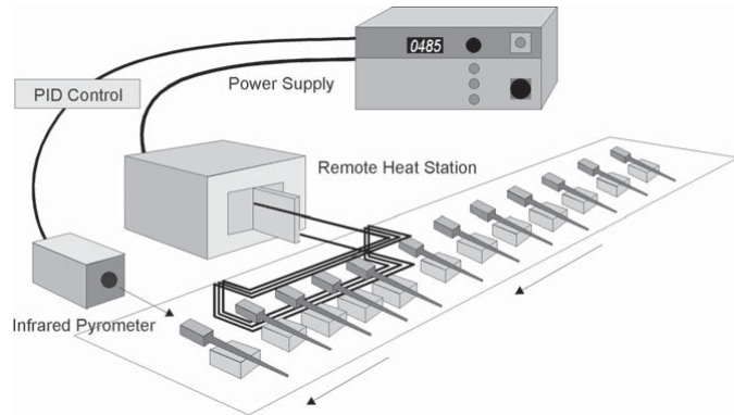
Figure 9: The Nova Star power supply's output is controlled by the infrared pyrometer's signal, forming a closed loop control system.
