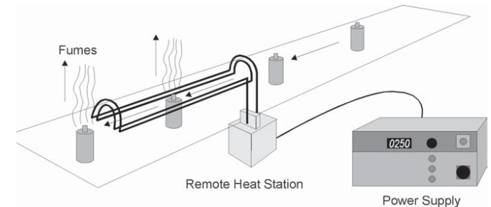
Figure 8: Both the low-voltage power supply and remote heat station can be located out of the path of the corrosive flux fumes produced by this soldering application.
