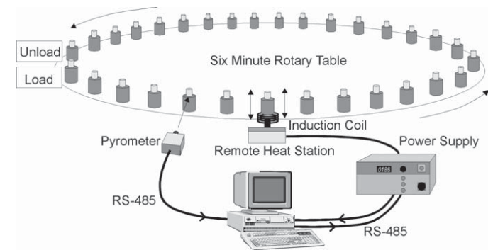
Figure 6: The computer instructs the power supply to deliver the required energy to heat the steel plug to 450° F.
