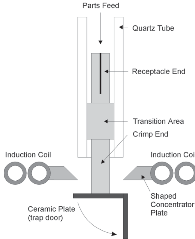
Figure 1: The crimp end of the copper connector is annealed with heat so that the metal is more easily formed around the wire. Precision Induction Heating
