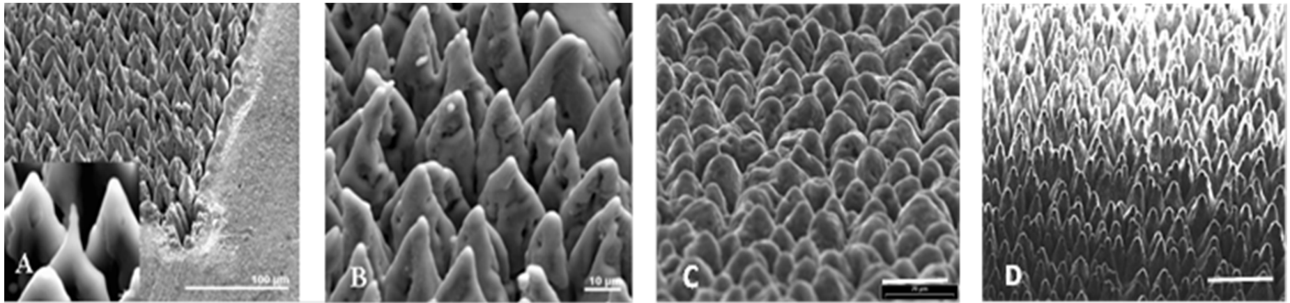
Figure 1. Scanning electron micrographs (SEM) of laser processed stainless steel (A), Ti (B), SiC ceramic(C) and SiN ceramic (D) showing fabricated micro-column arrays. Markers on (A), (B), (C), and (D) are 100, 10, 100, and 100 \mu\text{m} , respectively.
