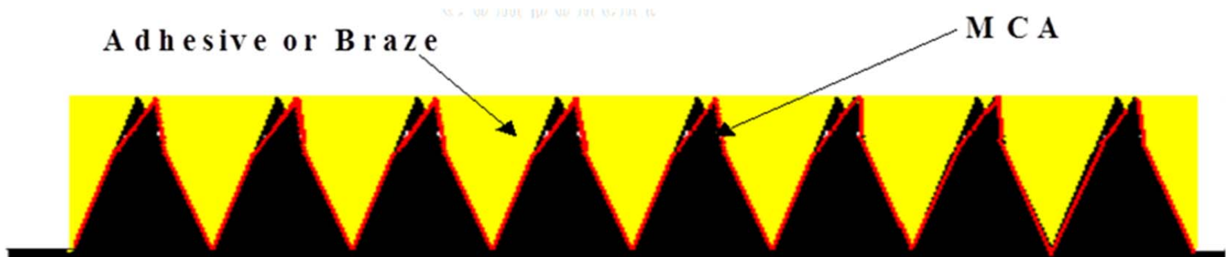
Figure 2. Micro-deformation of cones under shear stress in the presence of adhesive or braze.
