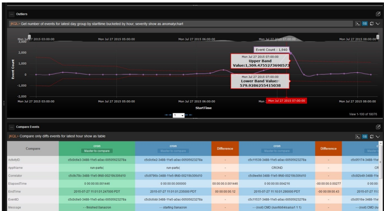
Figure 8: The Viewlet at the top shows an analysis of application events using Bollinger Bands and Exponential Moving Averages (EMAs). The Viewlet on the bottom is a comparison showing the differences between events.
