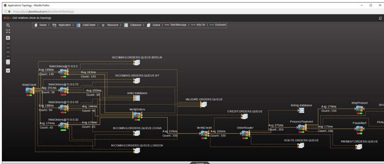
Figure 5: The Topology Viewlet above shows an automatically “stitched” transaction flow. It starts at the left with web browsers, then on to web applications, SQL databases, MQ Queues and more. No manual effort or modeling is required.
