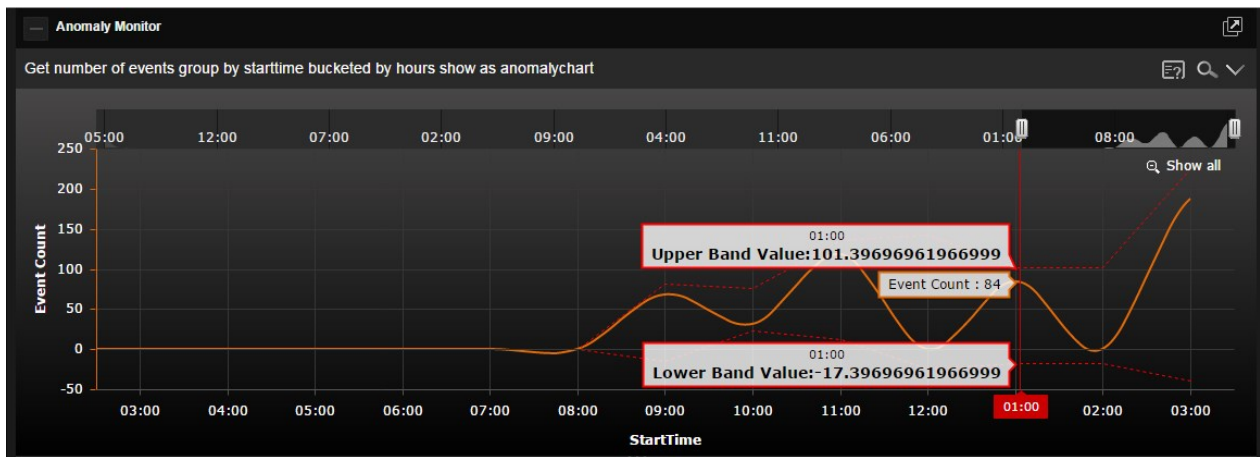
Figure 6: The above image shows how AutoPilot Insight automatically detects anomalies. The Anomaly Chart above uses Bollinger Bands and Exponential Moving Averages (EMA's) to auto-detect anomalies when an event crosses either the lower or upper bands. This is a self-maintaining analysis.
