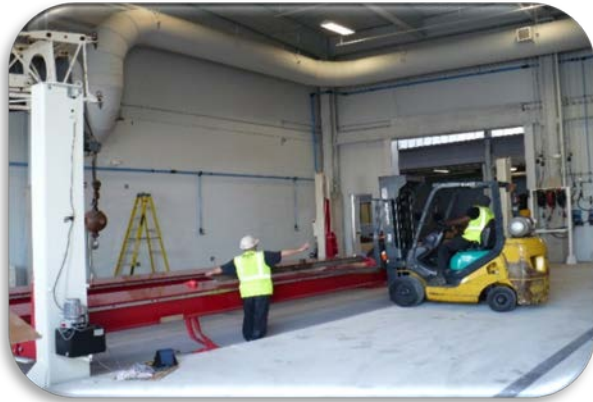
The ST 4600 can be installed on any suitable concrete floor
