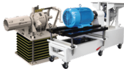
Power Test Electric Motor Testing Systems
