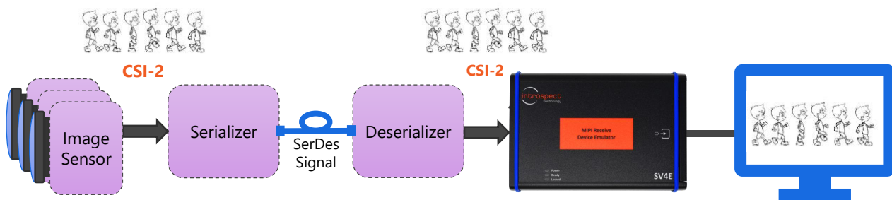
SV4E-CSI2-HDMI testing a complete multi-sensor automotive link
